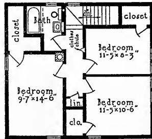
Second-floor Plan
